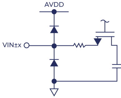
Figure 7. Equivalent Analog Input Circuit
