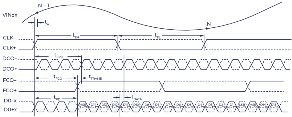
Figure 5. Word wise DDR, One-Lane, 1x Frame, 16-Bit Output Mode
