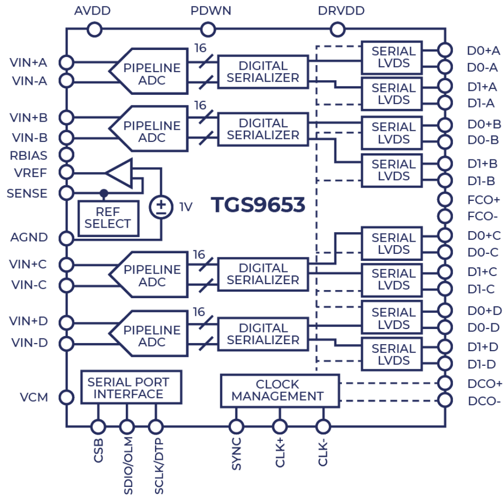
Figure 2. Block Diagram
