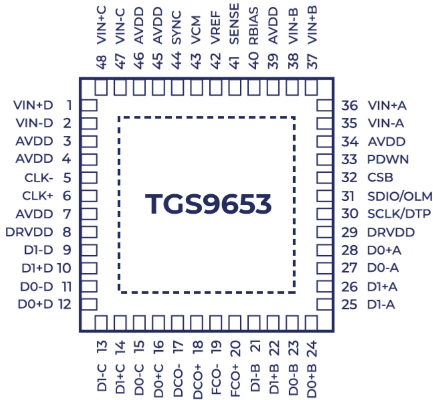
Figure 1. Pin Configuration
