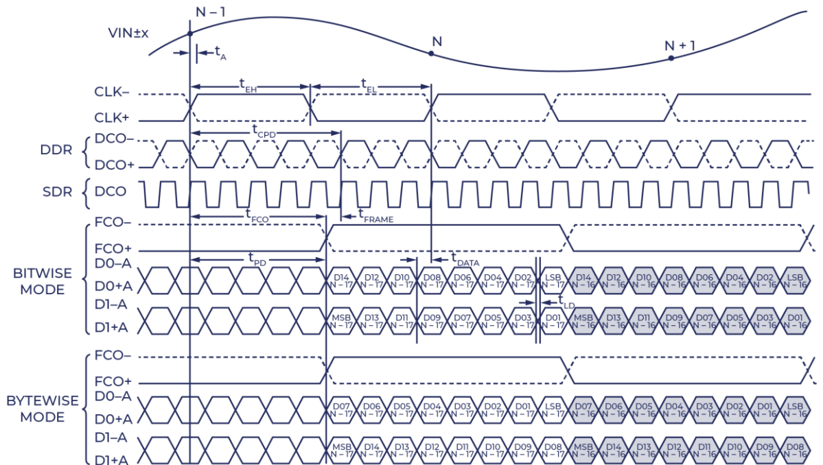
Figure 4. 16-Bit DDR/SDR, Two-Lane, 2x Frame Mode
