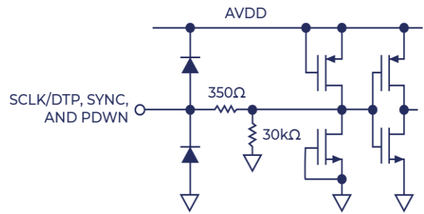
Figure 12. Equivalent SCLK/DTP, SYNC, and PDWN Input Circuit
