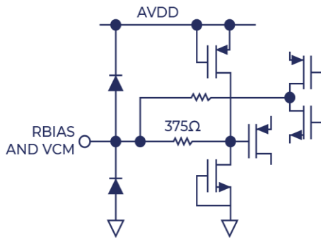
Figure 11. Equivalent RBIAS and VCM Circuit
