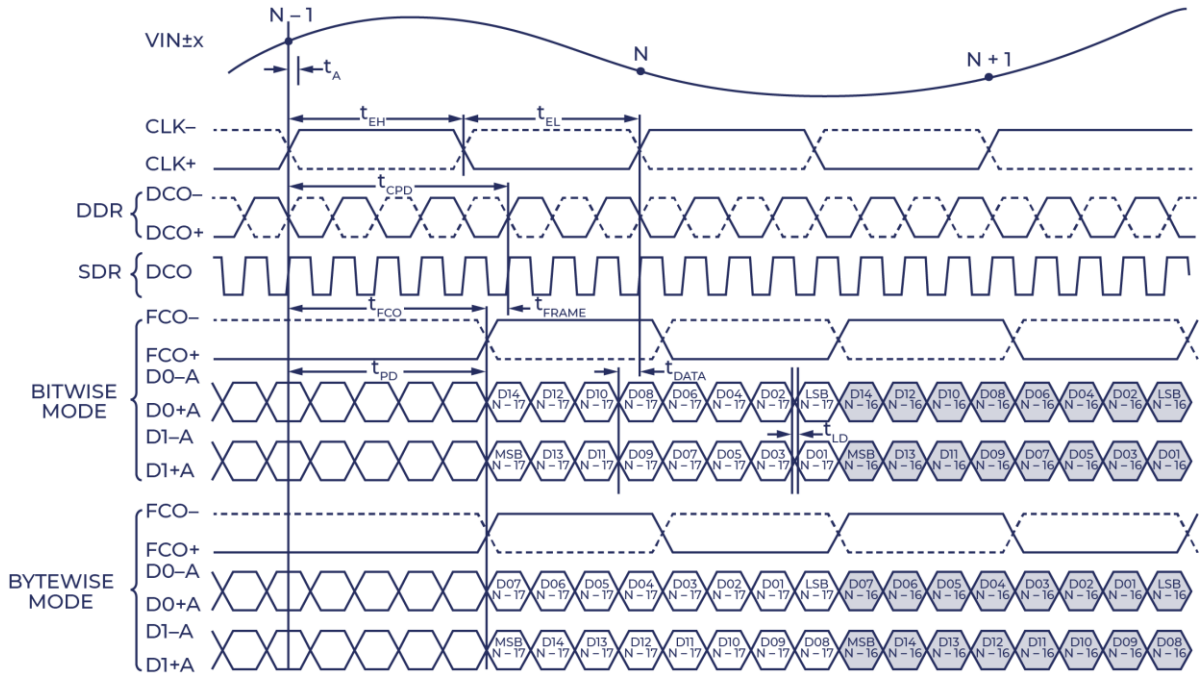
Figure 3. 16-Bit DDR/SDR, Two-Lane, 1x Frame Mode (Default)
