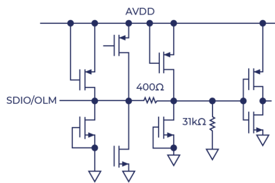
Figure 10. Equivalent SDIO/OLM Input Circuit
